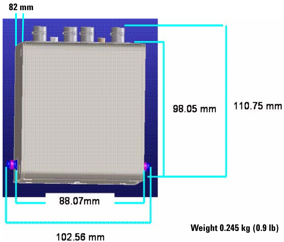
Figure 1 Dimensions
